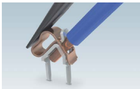
Spring-cage connection
