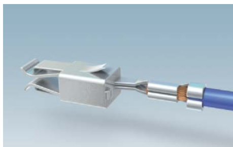
Crimp connection
